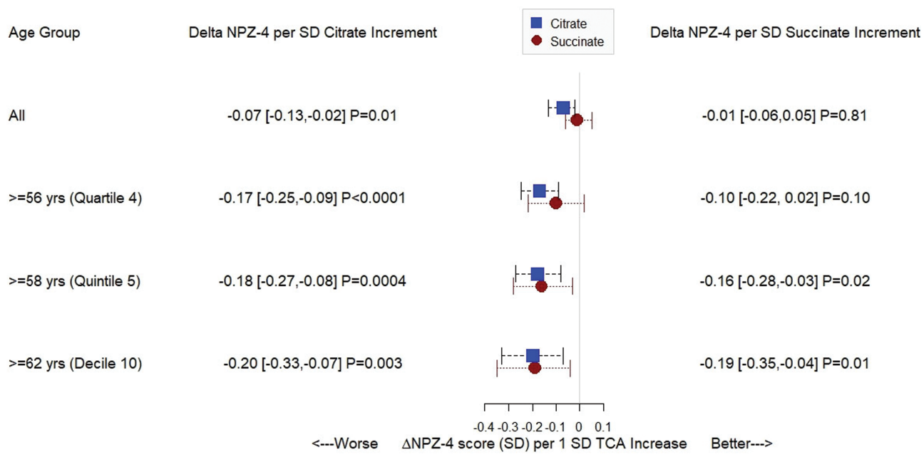
Figure 2. Association between time-updated NPZ-4 scores and 1 SD increase in plasma citrate and succinate concentrations overall, and for oldest 25th, 20th, and 10th percentiles. Symbols represent change in NPZ-4 score per 1 SD increase in entry TCA cycle metabolites in adjusted mixed effects linear models for time-updated NPZ-4 scores; error bars represent 95% confidence interval. Models adjusted for age, sex, race, education status, antiretroviral therapy duration, and time-updated CD4+ cell counts, plasma viral loads and study week. Abbreviation: SD, standard deviation; TCA, tricarboxylic acid.
