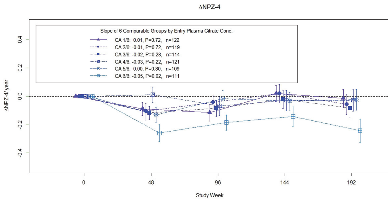
Figure 3. Change in NPZ-4 over time by entry plasma citrate concentrations in participants without NCI at entry. Symbols represent median NPZ-4 scores at each timepoint for participants grouped by entry plasma citrate concentration from lowest to highest. Error bars represent upper and lower 15th percentiles. The figure inset shows NPZ-4 slope over time for each of the 6 groups. Abbreviations: CA, citrate; NCI, neurocognitive impairment.
