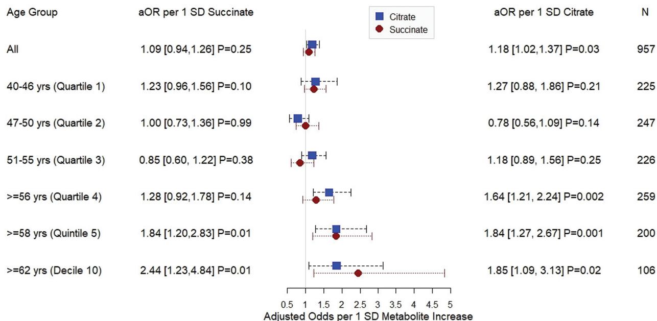
Figure 1. Association between prevalent NCI at entry and 1 SD increase in the plasma citrate and succinate concentration overall, by age-quartiles, and for oldest 20th and 10th percentiles. Symbols represent adjusted odds ratios for NCI per 1 SD increase in TCA cycle metabolite concentration in adjusted logistic regression models of prevalent NCI at entry; error bars represent 95% confidence intervals. Models adjusted for age, sex, race, education status, antiretroviral therapy duration, CD4+ cell count, and plasma viral load. Abbreviations: aOR, adjusted odds ratio; NCI, neurocognitive impairment; SD, standard deviation; TCA, tricarboxylic acid.
