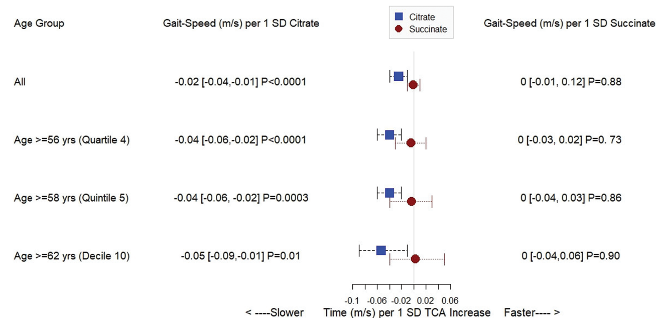
Figure 4. Association between time-updated gait speed and 1 SD increase in plasma citrate concentrations overall, and for oldest 25th, 20th, and 10th percentiles. Symbols represent effect on gait-speed (as m/s) for each 1 SD increase of entry TCA cycle metabolites in adjusted mixed effects linear models for time-updated gait speed; error bars represent 95% confidence interval. Models adjusted for age, sex, race, ART-duration, and time-updated CD4+ count, plasma viral load, and study week. Abbreviations: ART, antiretroviral therapy; SD, standard deviation; TCA, tricarboxylic acid.
