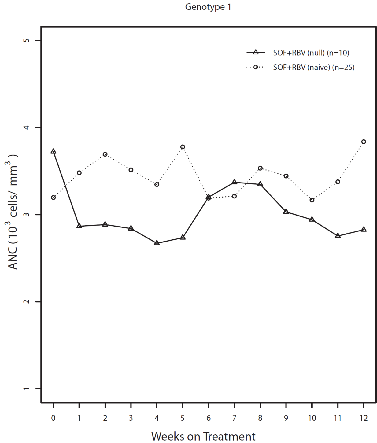
Figure S3B. Mean on-treatment absolute neutrophil counts over time in genotype 1 patients during treatment
